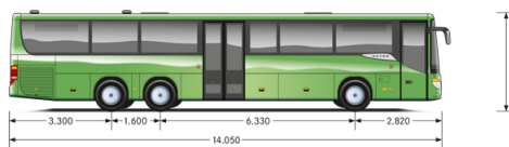
All dimensions in millimetres.
