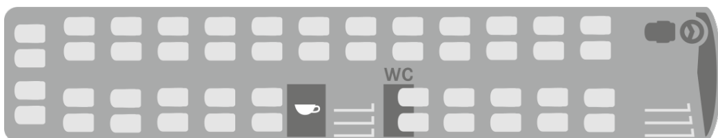
Variant 2 S 516 HD - 4 stars - 48 seats - Class 3 + WC + on-board kitchen
